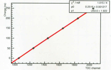
TDC RPC-170 No.005: Calibration 5 ch
