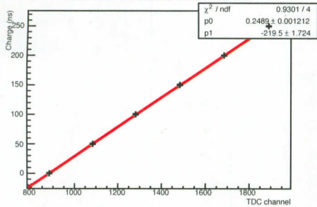
TDC RPC-170 No.005: Calibration 3 ch
