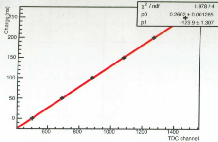
TDC RPC-060 No.061: Calibration 3 ch
