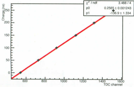
TDC RPC-060 No.061: Calibration 6 ch
