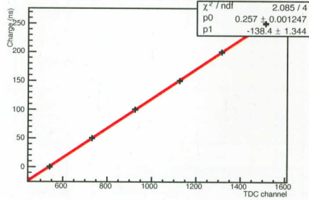
TDC RPC-060 No.061: Calibration 7 ch
