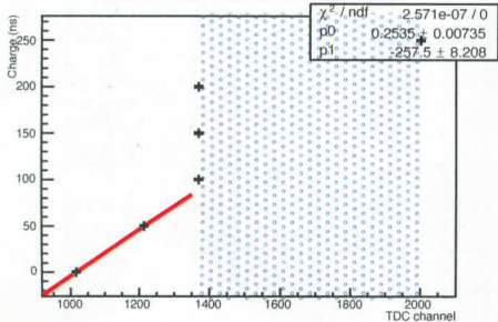
TDC RPC-170 No.005: Calibration 6 ch
