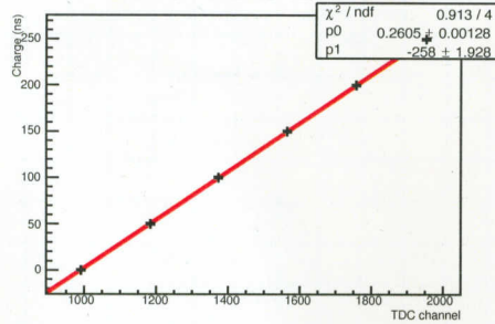
TDC RPC-170 No.005: Calibration 4 ch
