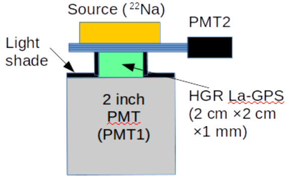
Fig. 1. This is the setting of experiment. PMT1 is the trigger detector.
