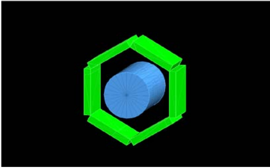
Fig. 2. This is Overall view of simulation in GEANT4. Green blocks are La-GPS scintillators, and a blue tube is human.
