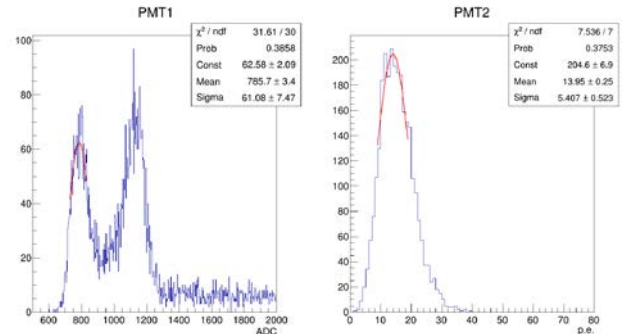
Fig. 5. This is a graph of the number of p.e. in 290-390 keV gamma rays with 6 WLSF sheets.
