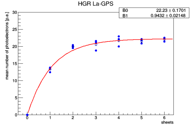
Fig. 3. This is a graph of relationship between the number of WLSF sheets and the number of p.e. in 511-keV gamma rays.
