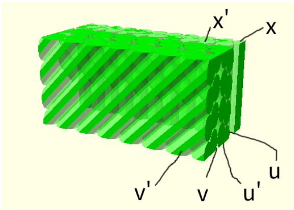
Fig. 3. Construction of scintillating fibre traker.
