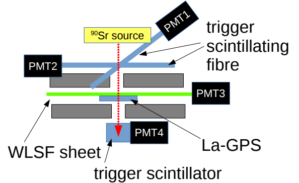
Fig. 4. Setup of the experiment
