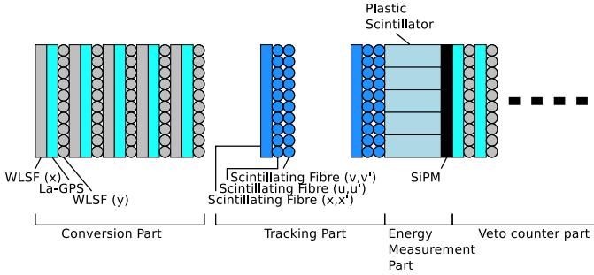
Fig. 2. A schematic diagram of the system
