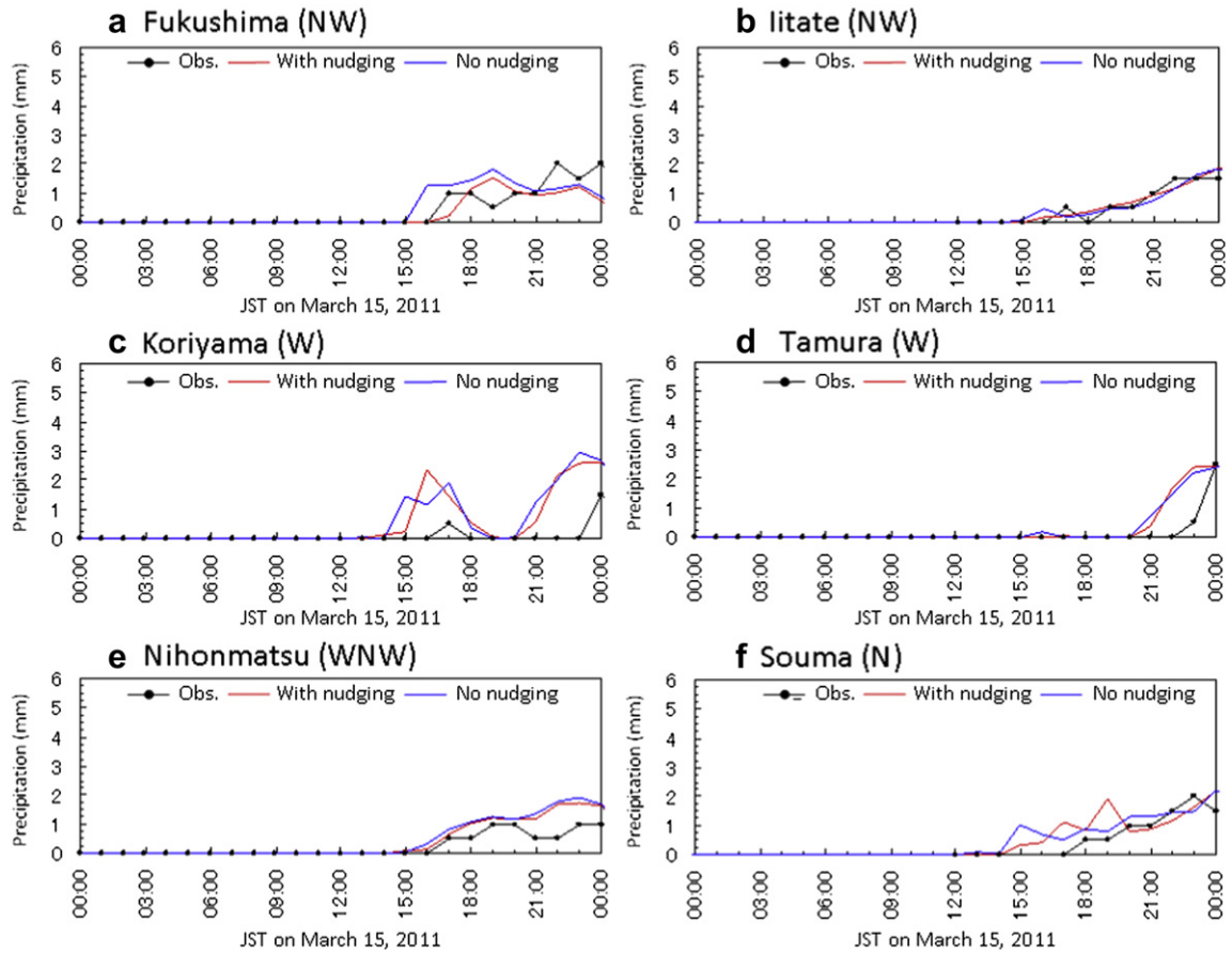
Fig. 4. Comparisons between MM5 calculations with/without nudging (lines) and observations (black lines with dots) for precipitation at the surface weather stations located at the northwest (NW), west (W), west-northwest (WNW), and north (N) directions from FNPP1.
