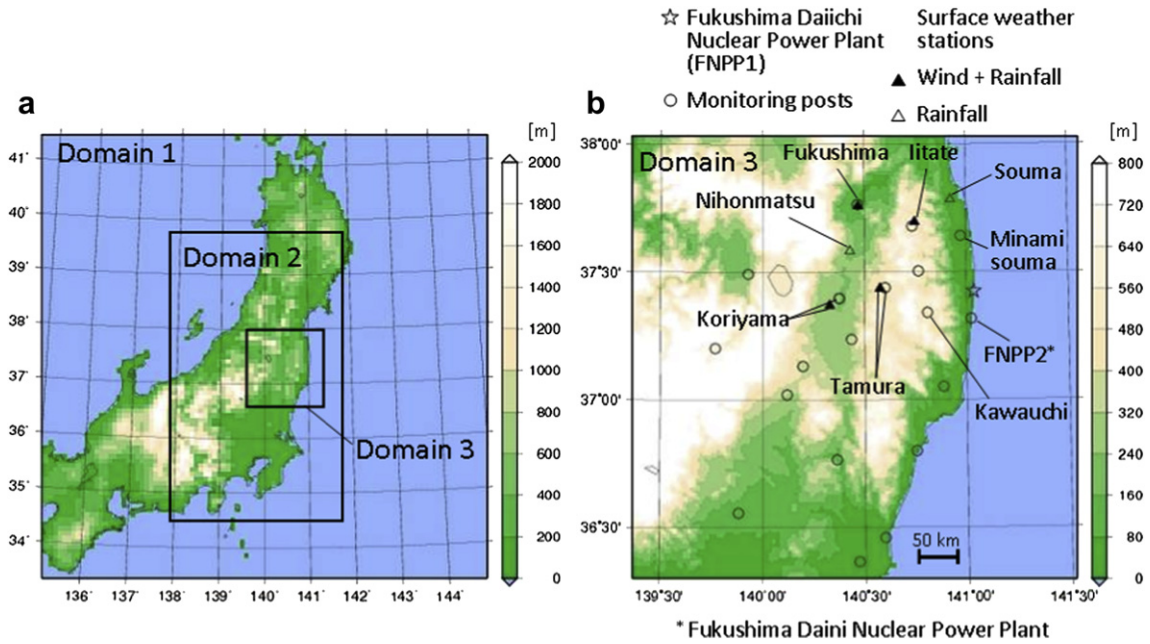
Fig. 2. Topography and simulation domain size of (a) Domain 1 and (b) 3 in MM5 and GEARN. Plots with labels in (b) show the environmental data used to reproduce the meteorological fields and radiological events by WSPEEDI-II. Other plots without labels represent the monitoring posts for comparisons in spatial patterns of air dose rate between observations and calculations by GEARN.
