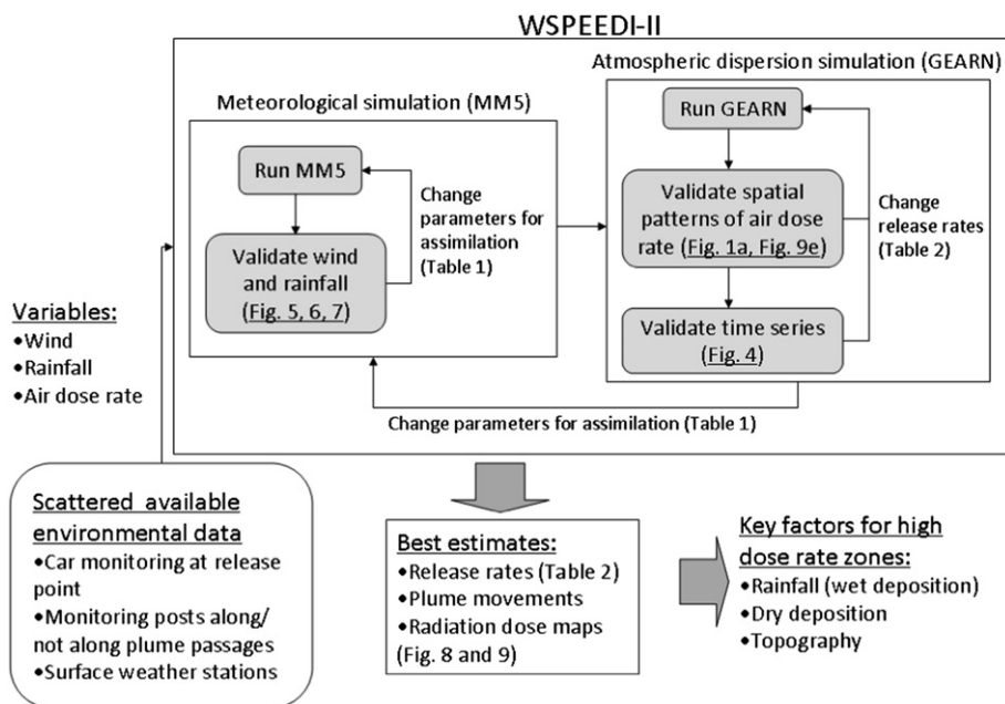
Fig. 6. Procedure for reconstruction of atmospheric dispersion of radionuclides in Fukushima Dai-ichi nuclear reactor accident using Worldwide Version of System for Prediction of Environmental Emergency Dose Information (WSPEEDI-II).
