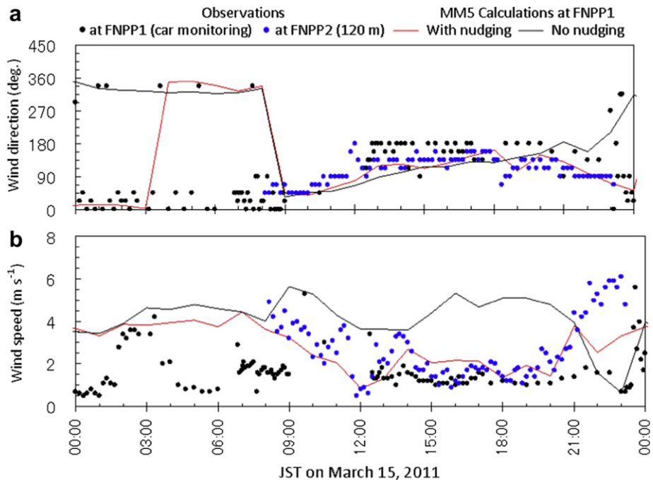
Fig. 5. Temporal changes in (a) wind direction and (b) speed in observations (circles) and MM5 calculations (lines) at FNPP1 and FNPP2.
