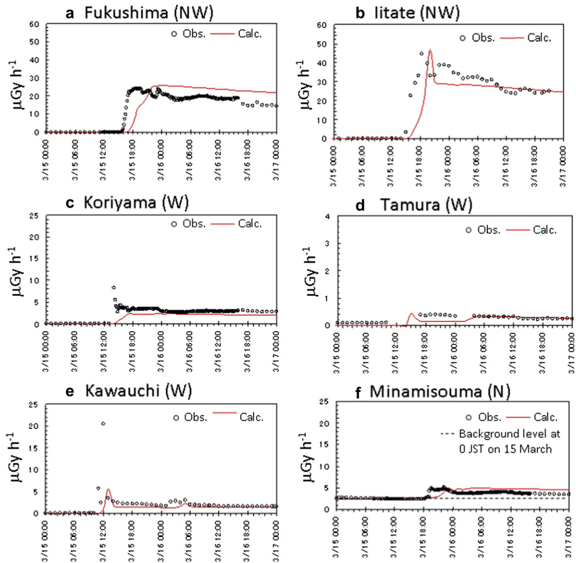
Fig. 7. Temporal changes of calculated (lines) and observed (circles) air dose rates at monitoring posts located at the northwest (NW), west (W), west-northwest (WNW), and north (N) directions from FNPP1.
