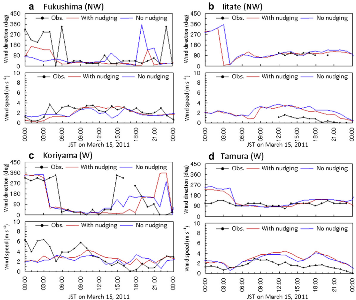
Fig. 3. Comparisons between MM5 calculations with/without nudging (lines) and observations (circles) for wind direction and speed at the surface weather stations located at the northwest (NW) and west (W) directions from FNPP1.
