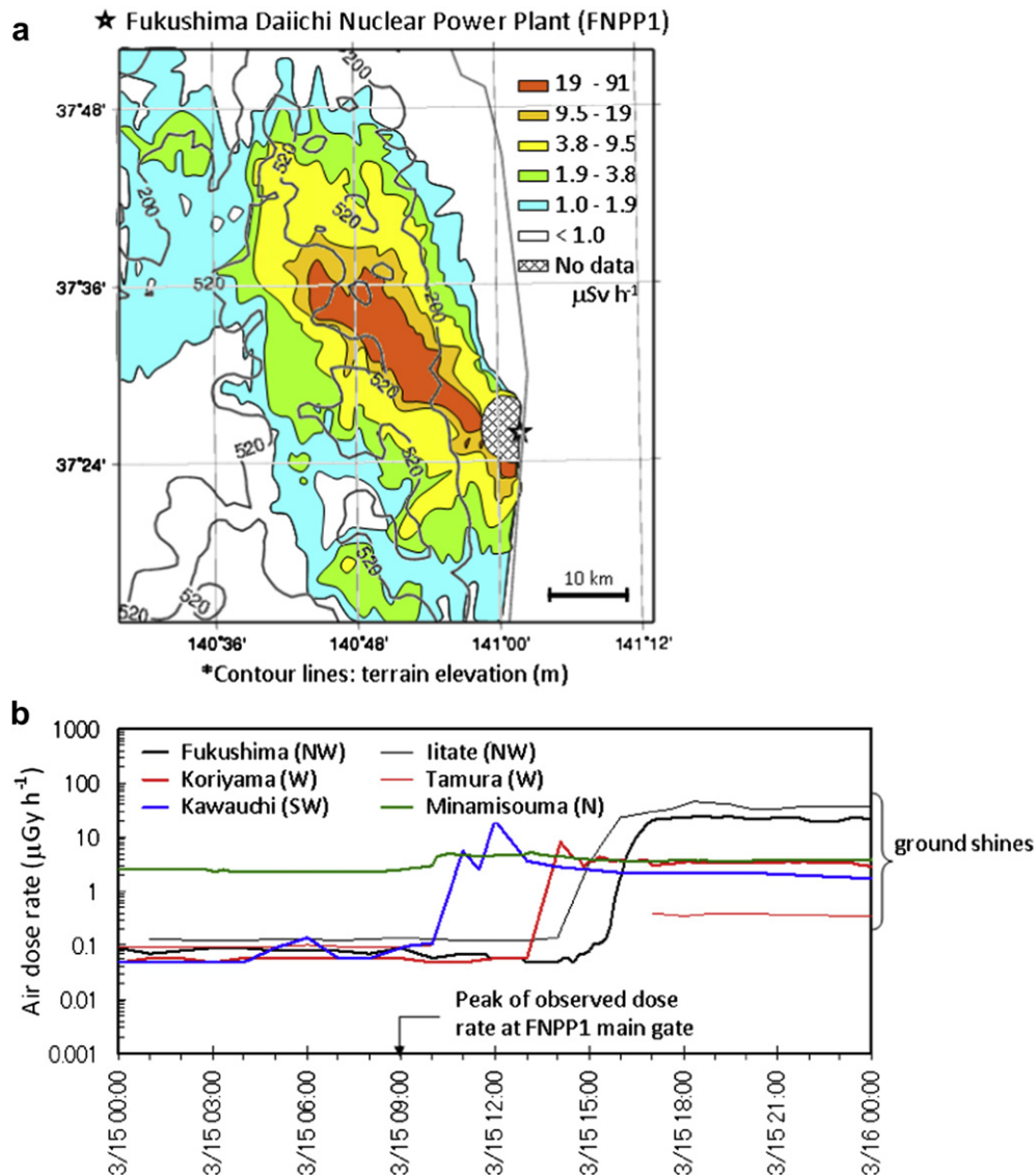
Fig. 1. Observed ground-level air dose rates in Fukushima prefecture by (a) aerial measurements (MEXT and DOE, 2011, reproduced from the authors) and (b) monitoring posts (Fukushima prefecture, 2011a and b). Words in parentheses in (b) show the direction of the locations from FNPP1.
