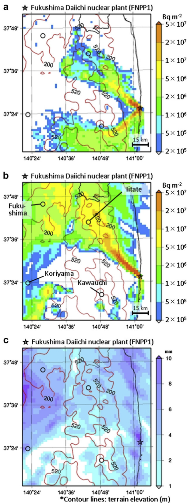
Fig. 10. Spatial distributions of (a) calculated dry and (b) wet deposition and (c) precipitation accumulated from 0 to 21 JST on March 15, 2011.
