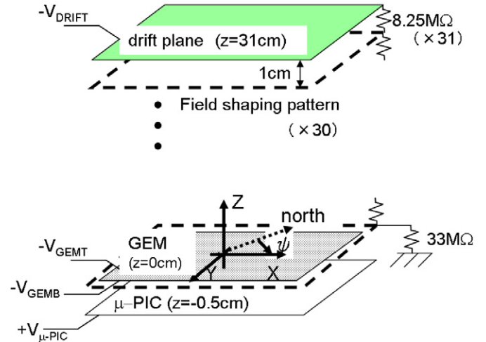
Fig. 1. Schematic drawings of the \mu -TPC. \mu -PIC and the GEM are set horizontally.
