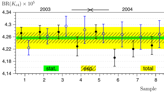
Fig. 5. K_{e4} branching ratio for eight statistically independent samples and both kaon charges. The hatched band shows the experimental error ( \sigma_{\text{exp}} = \sigma_{\text{stat}} \oplus \sigma_{\text{syst}} ). The total error (shaded band) includes the external error. The fit \chi^2 is 15.85 for 15 degrees of freedom when including the time-dependent errors only. Full symbols correspond to K^+ results and empty symbols to K^- results.
