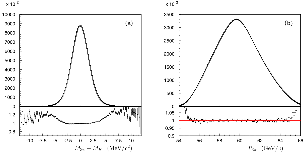
Fig. 3. Distributions of the reconstructed M_{3\pi} invariant mass (a) and the reconstructed kaon momentum (b) for the normalization K_{3\pi} candidates within the final selection. Data are shown as symbols and simulation normalized to data as histograms. The lower plots are the ratios of the distributions (data/simulation) displayed in the upper plots.
