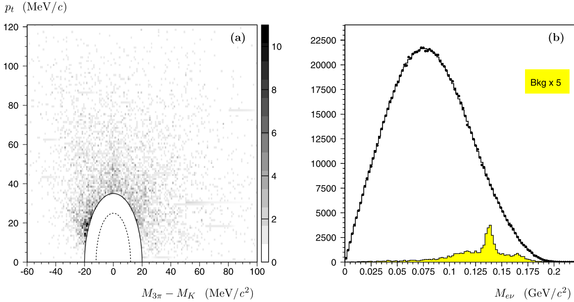
Fig. 2. (a) Reconstructed (M_{3\pi}, p_t) plane for the K_{e4} background estimated from WS events. The elliptic cuts used in the WS selection (solid line) and normalization (dashed line) selections are shown. (b) Reconstructed dilepton invariant mass for K_{e4} events. Data are shown as symbols, simulation as histogram and background events (scaled by a factor of 5 to be visible) as shaded area.
