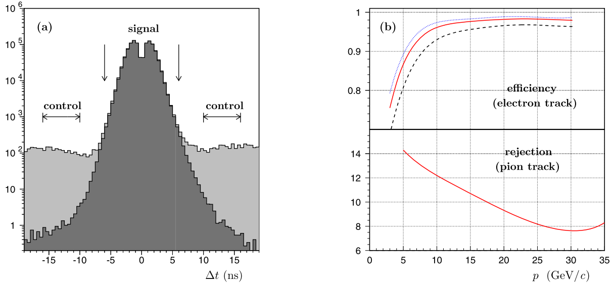
Fig. 4. (a) Normalized distribution of the time difference between the time of each vertex track and their average for K_{e4} (light shaded area) and K_{3\pi} (dark shaded area) candidates. The vertical arrows indicate the signal time window. The horizontal arrows indicate the two control regions. Only the time difference of the track with the largest \Delta t absolute value is plotted. (b) Efficiency of the linear discriminant variable as a function of momentum for electron tracks (top curves). The solid line corresponds to the cut value of 0.90 applied in this analysis. The lower dashed line corresponds to the cut value of 0.95 and the upper dotted line to the cut value of 0.85. For illustration, the pion track rejection (bottom curve) is displayed for the cut value of 0.90.
