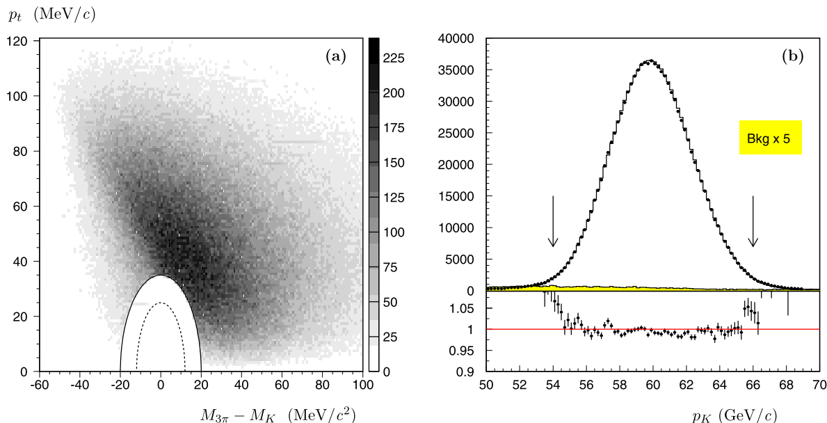
Fig. 1. (a) Reconstructed (M_{3\pi}, p_t) plane for the K_{e4} signal candidates. The elliptic cuts used in the signal (solid line) and normalization (dashed line) selections are shown. (b) Reconstructed kaon momentum from signal events for data after background subtraction (symbols), simulation normalized to data (histogram) and background events (scaled by a factor of 5 to be visible) as shaded area. The arrows point to the kaon momentum cuts values. The lower plot is the ratio of the two spectra (data/simulation) displayed in the upper plot.
