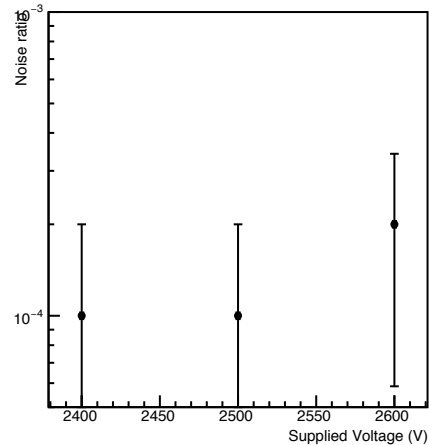
Noise ratio: H1161 2"PMT Arr'y Z02320
